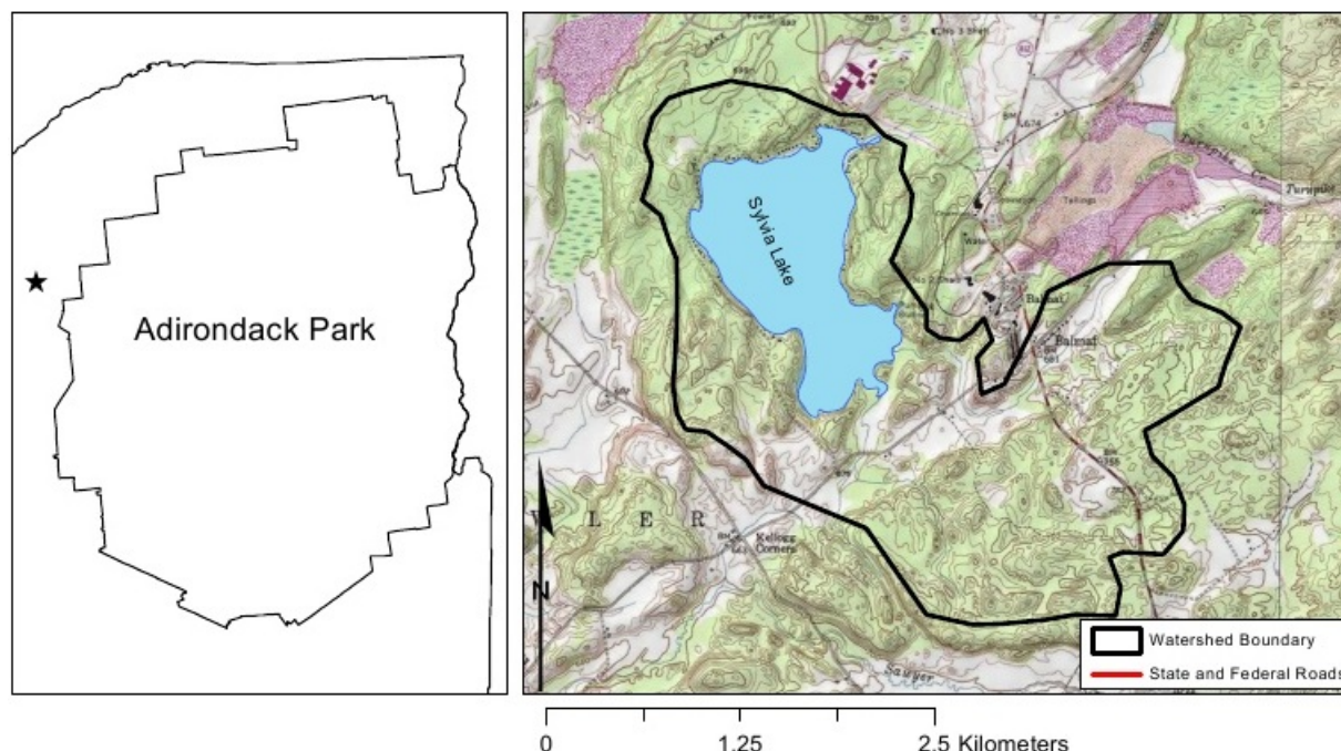
Figure 2. Location and watershed for Sylvia Lake.
