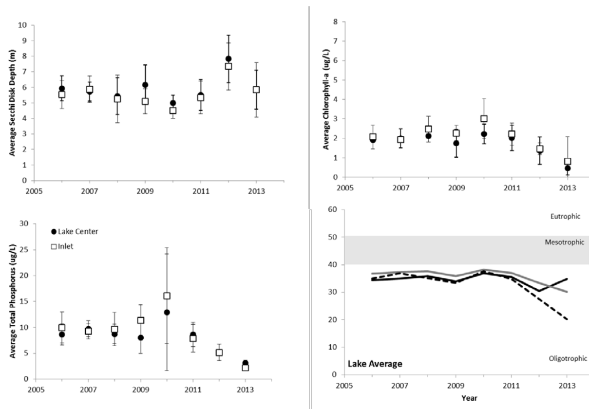
Figure 3. The annual average values of epilimnetic trophic indicators of Sylvia Lake at the inlet and the lake center 2006-2013. (A) Secchi disk transparency, (B) total phosphorus concentration, (C) chlorophyll-a concentration, and (D) Carlson's Trophic State Index. Vertical bars represent one standard deviation of the mean. Significant trends ( P < 0.05 ) are noted with a trend line.
