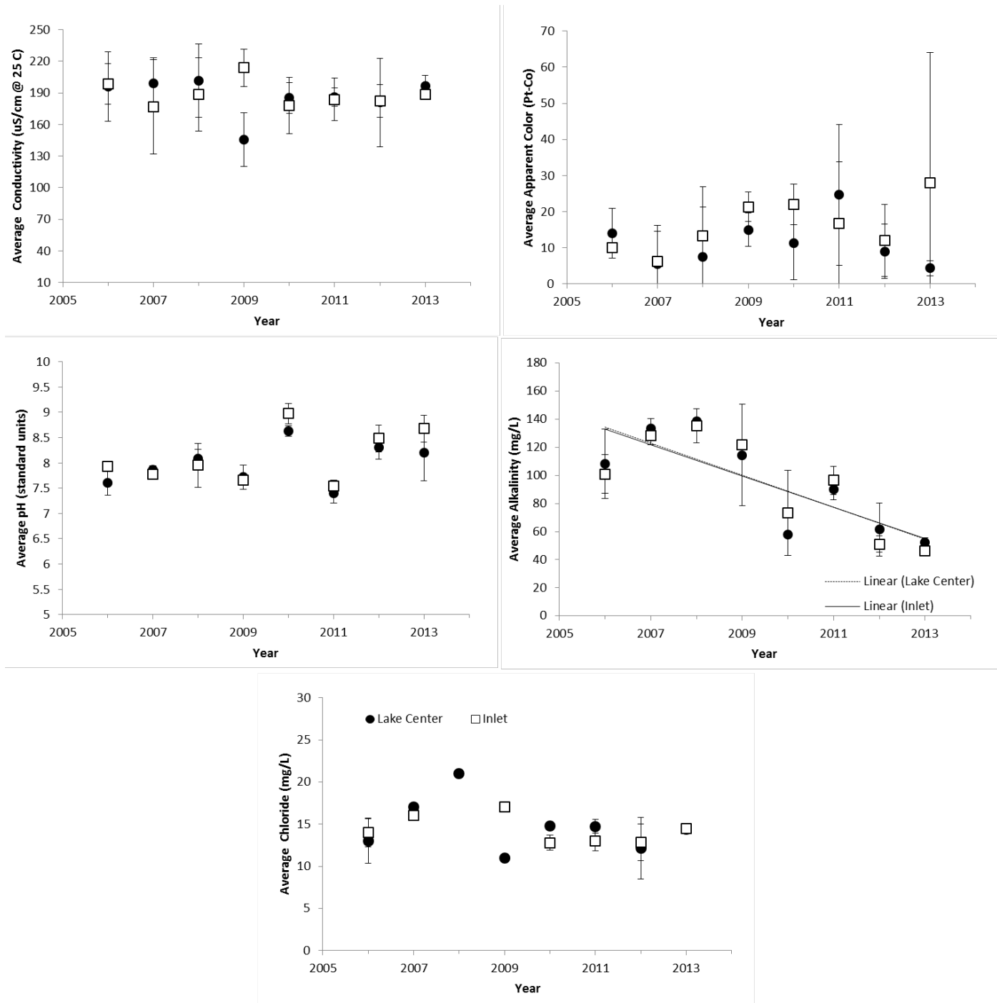
Figure 4. The annual average values of water quality indicators of Sylvia Lake at the inlet and the lake center 2006-2013. (A) Specific lab conductivity @ 25°C, (B) apparent color, (C) pH, (D) total alkalinity, and (E) chloride concentration. Vertical bars represent one standard deviation of the mean. Significant trends ( P < 0.05 ) are noted with a trend line.
