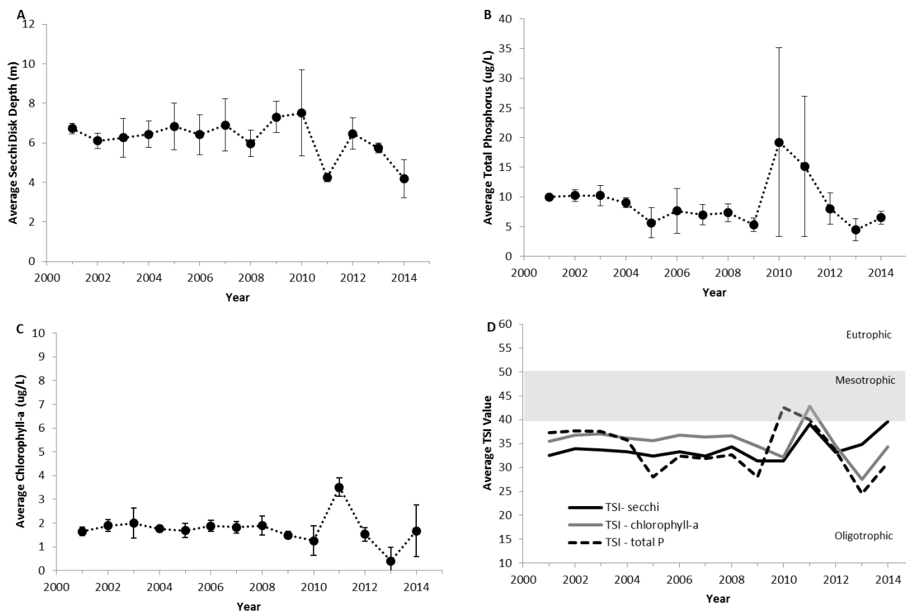
Figure 3. The annual average values of epilimnetic trophic indicators of Hoel Pond, 2001-2014. (A) Secchi disk transparency, (B) total phosphorus concentration, (C) chlorophyll-a concentration, and (D) Carlson's Trophic Status Index. Vertical bars represent one standard deviation of the mean. Significant trends ( P \leq 0.05 ) are noted with a trend line.
