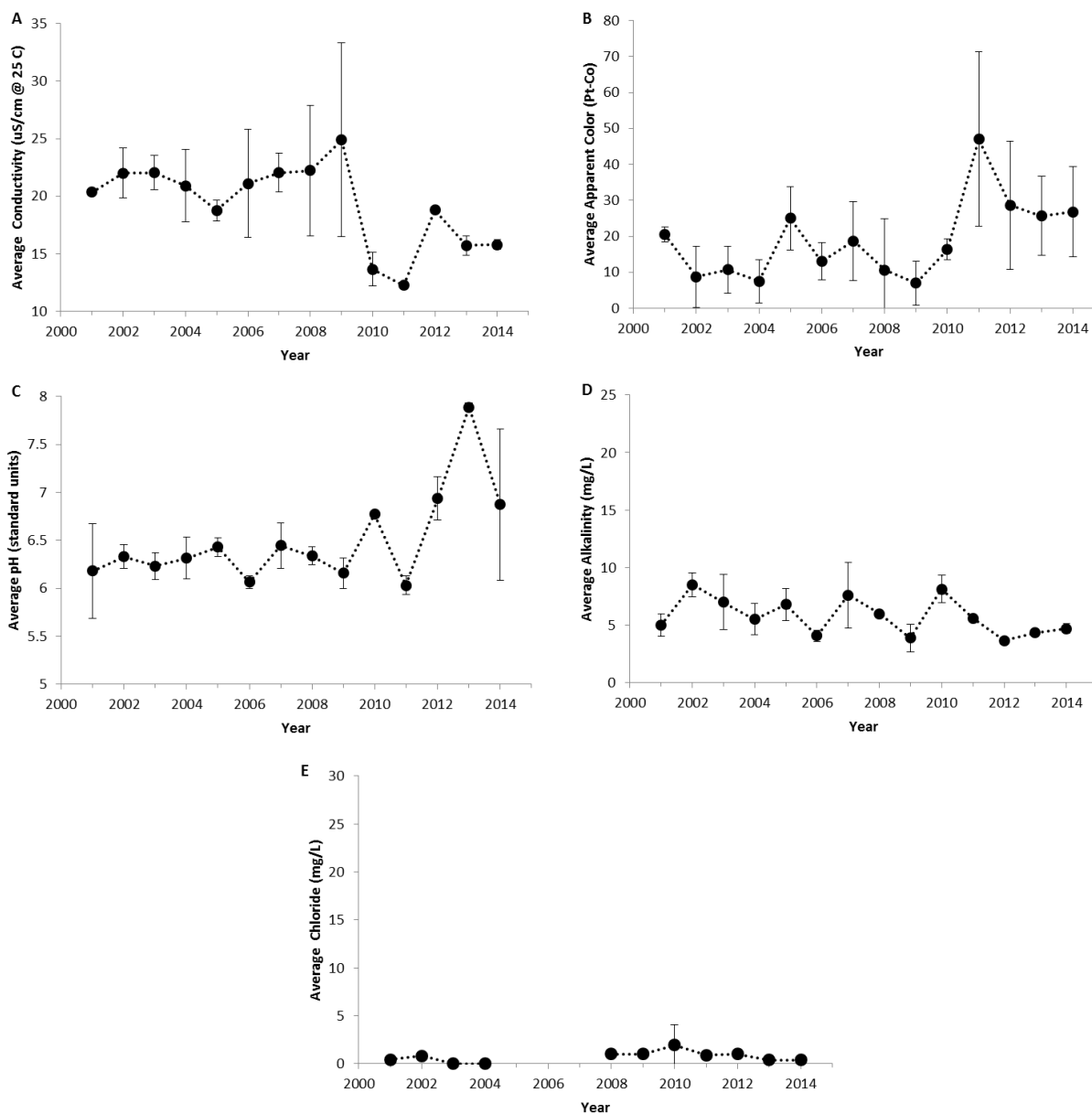
Figure 4. The annual average values of water quality indicators of Hoel Pond, 2001-2014. (A) Specific lab conductivity @ 25 C, (B) apparent color, (C) pH, (D) total alkalinity, and (E) chloride. Vertical bars represent one standard deviation of the mean. Significant trends ( P \leq 0.05 ) are noted with a trend line.
