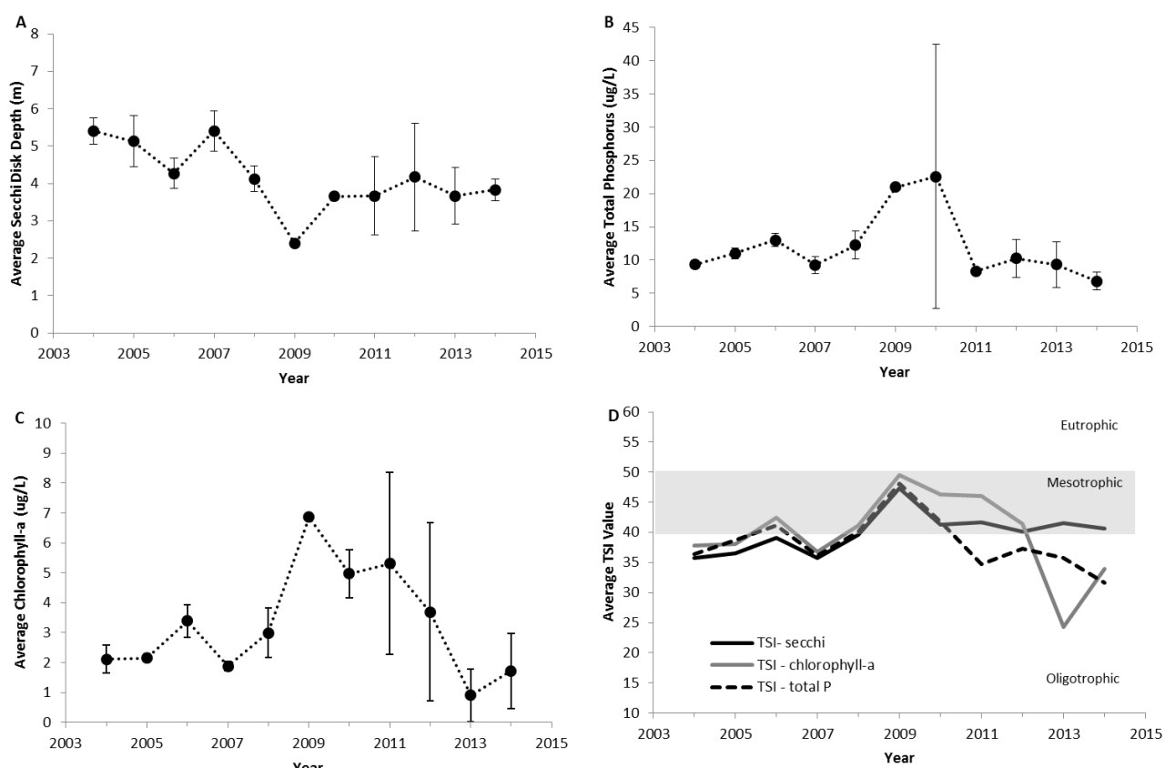
Figure 3. The annual average values of epilimnetic trophic indicators of Indian Lake, 2004-2014. (A) Secchi disk transparency, (B) total phosphorus concentration, (C) chlorophyll-a concentration, and (D) Carlson's Trophic Status Index. Vertical bars represent one standard deviation of the mean. Significant trends ( P \leq 0.05 ) are noted with a trend line.
