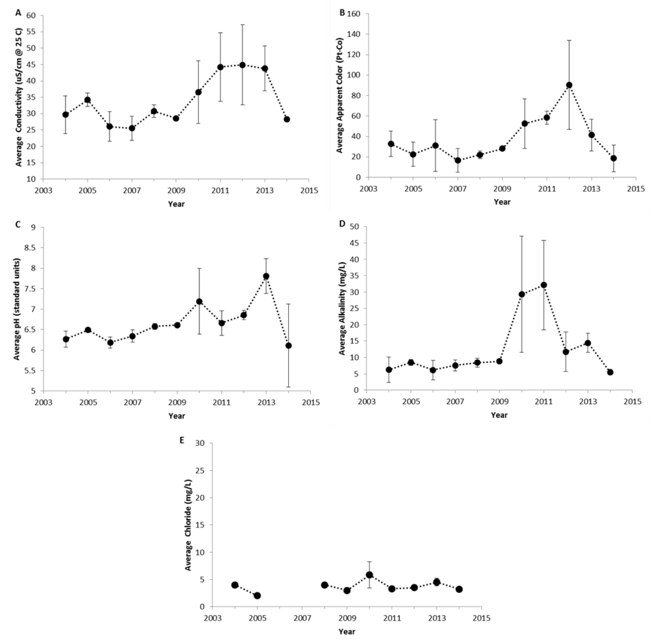
Figure 4. The annual average values of water quality indicators of Indian Lake, 2004-2014. (A) Specific lab conductivity @ 25 C, (B) apparent color, (C) pH, (D) total alkalinity, and (E) chloride. Vertical bars represent one standard deviation of the mean. Significant trends ( P \leq 0.05 ) are noted with a trend line.
