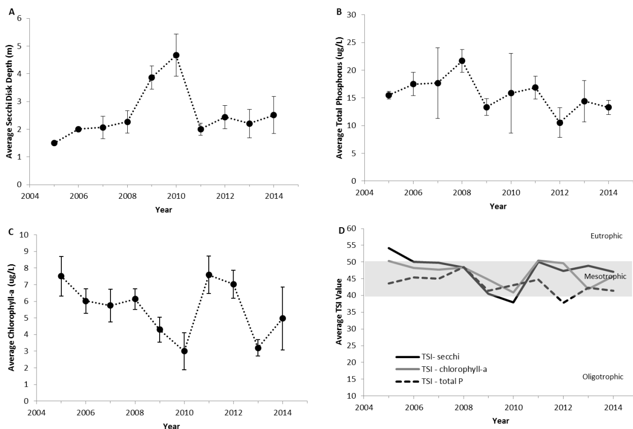
Figure 3. The annual average values of epilimnetic trophic indicators of Indian Lake, 2005-2014. (A) Secchi disk transparency, (B) total phosphorus concentration, (C) chlorophyll-a concentration, and (D) Carlson's Trophic Status Index. Vertical bars represent one standard deviation of the mean. Significant trends ( P \leq 0.05 ) are noted with a trend line.
