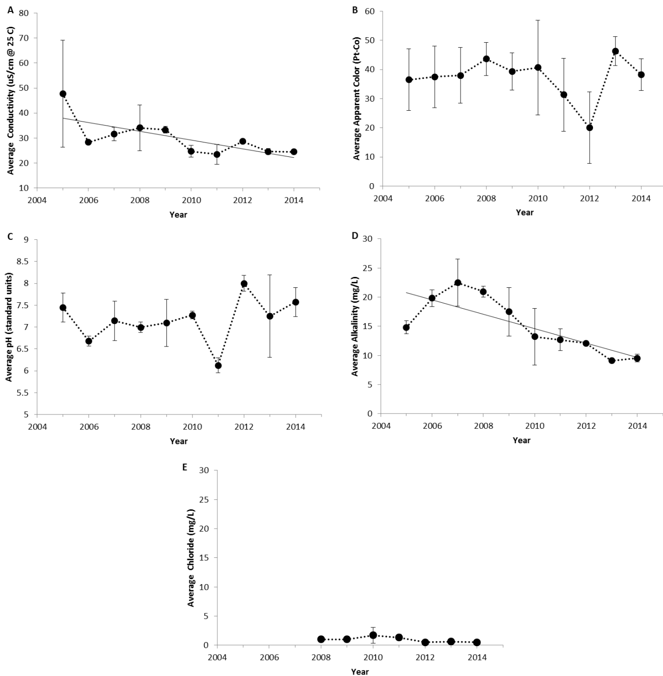
Figure 4. The annual average values of water quality indicators of Indian Lake, 2005-2014. (A) Specific lab conductivity @ 25 C, (B) apparent color, (C) pH, (D) total alkalinity, and (E) chloride. Vertical bars represent one standard deviation of the mean. Significant trends ( P \leq 0.05 ) are noted with a trend line.
