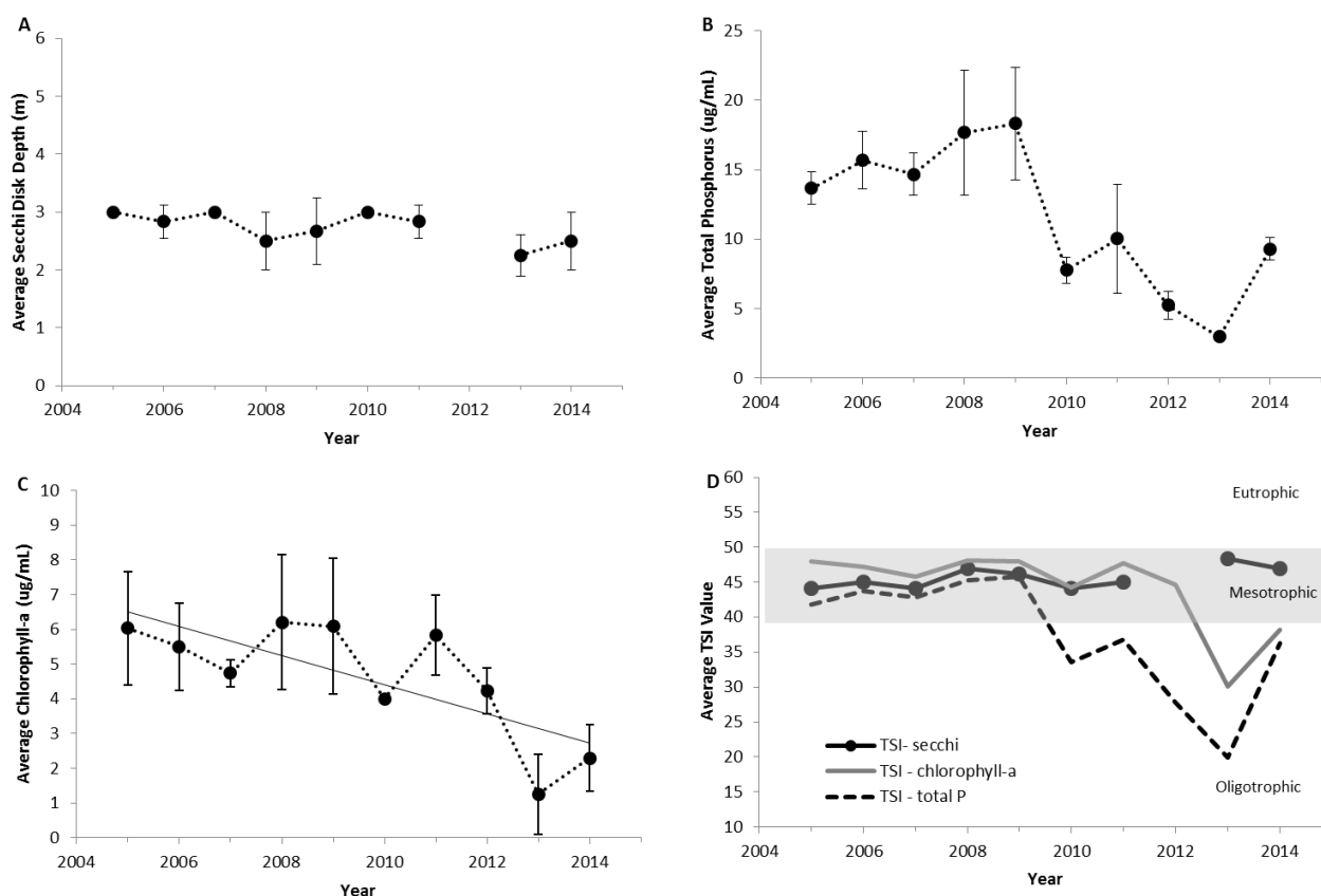
Figure 3. The annual average values of epilimnetic trophic indicators of Abanakee Lake, 2005-2014. (A) Secchi disk transparency, (B) total phosphorus concentration, (C) chlorophyll-a concentration, and (D) Carlson's Trophic Status Index. Vertical bars represent one standard deviation of the mean. Significant trends ( P \leq 0.05 ) are noted with a trend line.
