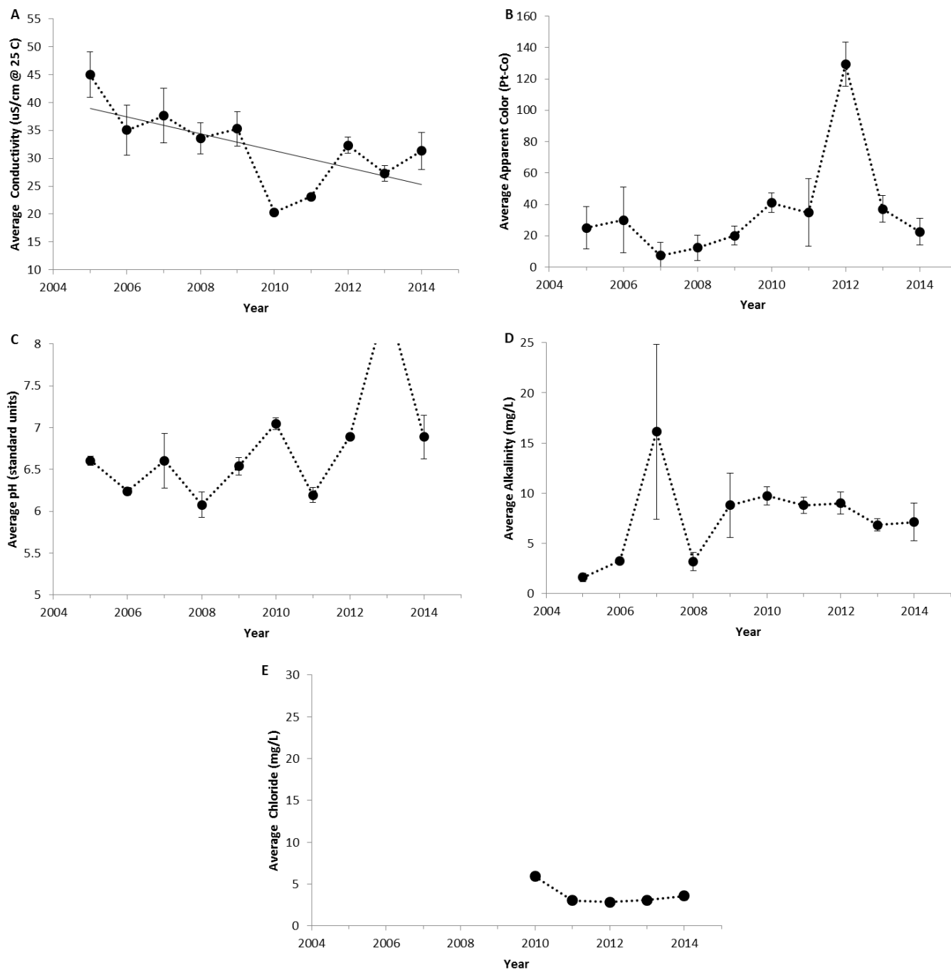
Figure 4. The annual average values of water quality indicators of Abanakee Lake, 2005-2014. (A) Specific lab conductivity @ 25 C, (B) apparent color, (C) pH, (D) total alkalinity, and (E) chloride. Vertical bars represent one standard deviation of the mean. Significant trends ( P \leq 0.05 ) are noted with a trend line.
