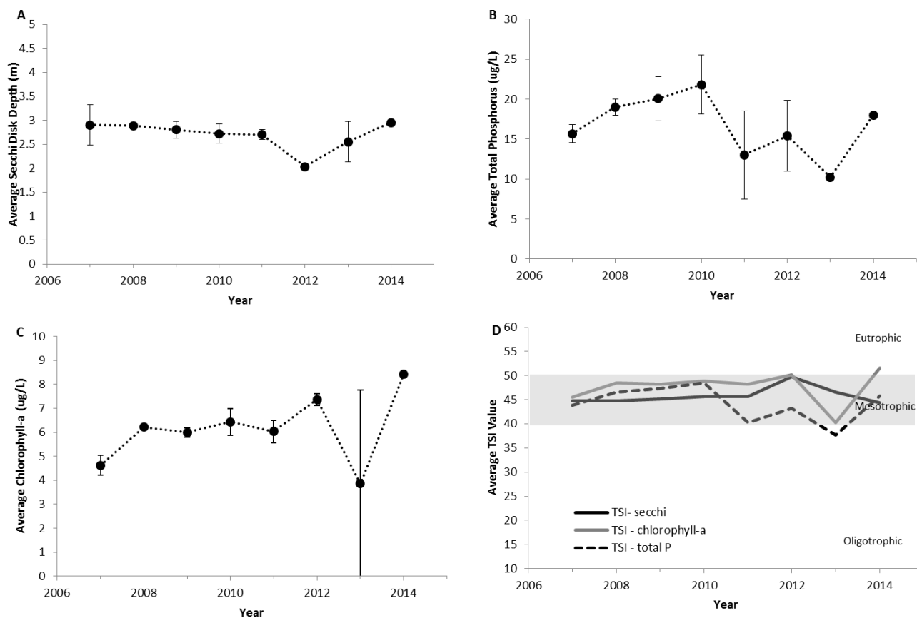
Figure 3. The annual average values of epilimnetic trophic indicators of Lake Adirondack, 2007-2014. (A) Secchi disk transparency, (B) total phosphorus concentration, (C) chlorophyll-a concentration, and (D) Carlson's Trophic Status Index. Vertical bars represent one standard deviation of the mean. Significant trends ( P \leq 0.05 ) are noted with a trend line.
