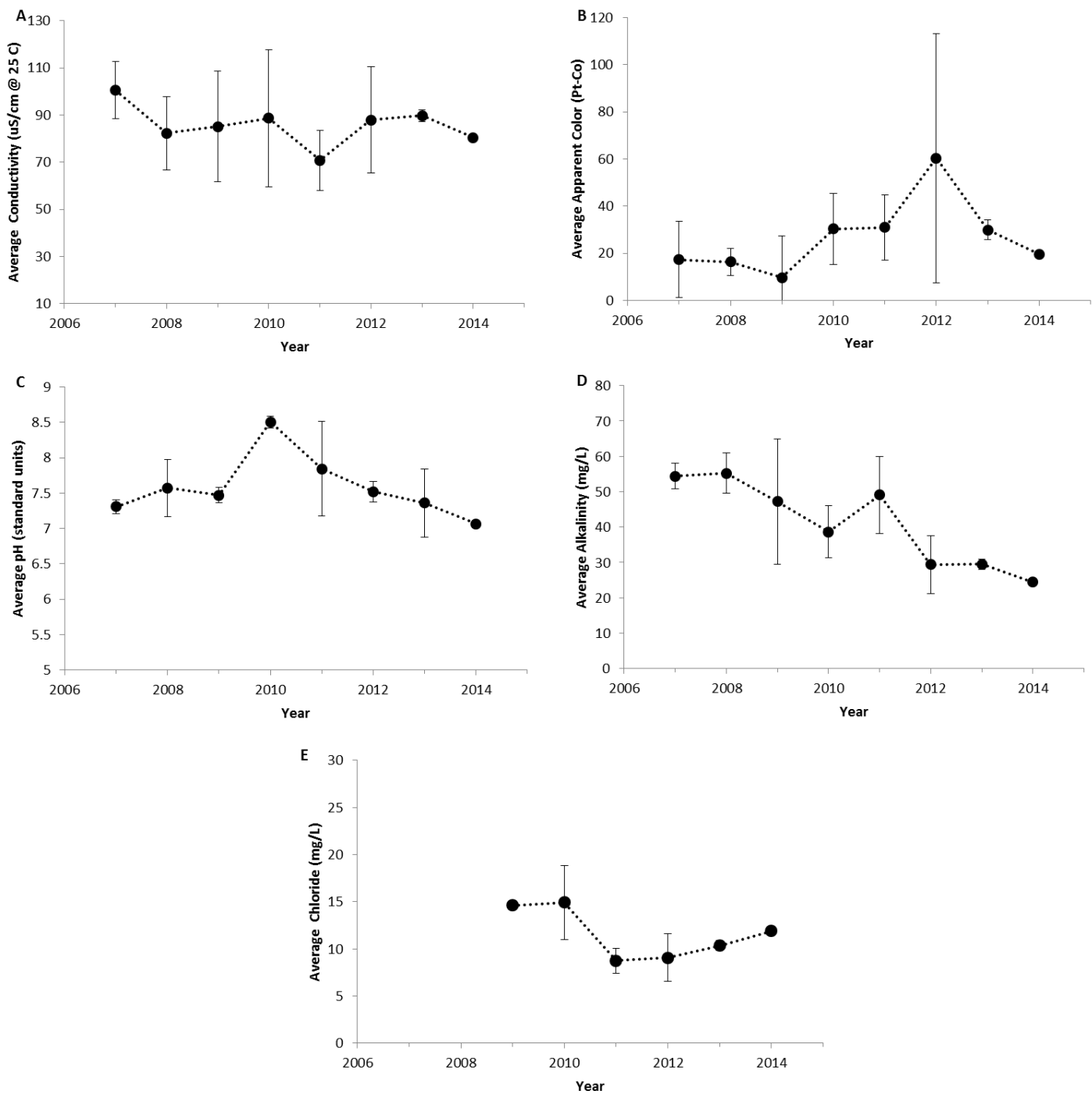
Figure 4. The annual average values of water quality indicators of Lake Adirondack, 2007-2014. (A) Specific lab conductivity @ 25 C, (B) apparent color, (C) pH, (D) total alkalinity, and (E) chloride. Vertical bars represent one standard deviation of the mean. Significant trends ( P \leq 0.05 ) are noted with a trend line.
