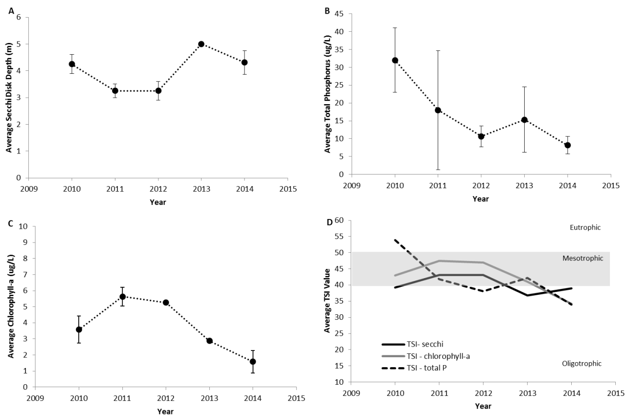
Figure 3. The annual average values of epilimnetic trophic indicators of Lake Titus, 2010-2014. (A) Secchi disk transparency, (B) total phosphorus concentration, (C) chlorophyll-a concentration, and (D) Carlson's Trophic Status Index. Vertical bars represent one standard deviation of the mean. Significant trends ( P \leq 0.05 ) are noted with a trend line.
