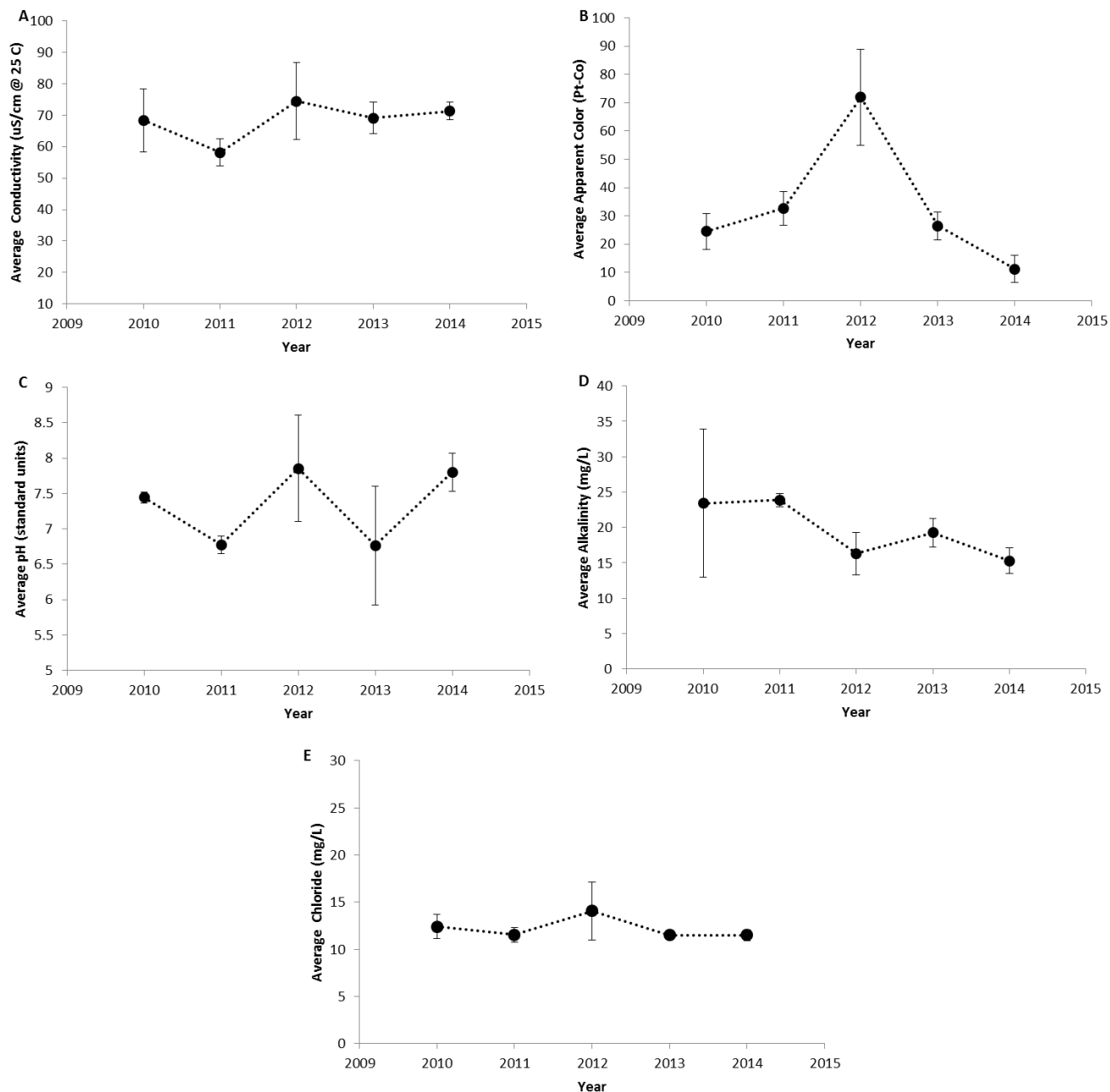
Figure 4. The annual average values of water quality indicators of Lake Titus, 2010-2014. (A) Specific lab conductivity @ 25 C, (B) apparent color, (C) pH, (D) total alkalinity, and (E) chloride. Vertical bars represent one standard deviation of the mean. Significant trends ( P \leq 0.05 ) are noted with a trend line.
