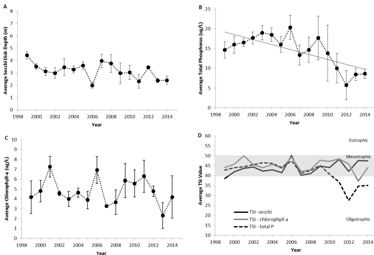
Figure 3. The annual average values of epilimnetic trophic indicators of Little Long Lake, 1999-2014. (A) Secchi disk transparency, (B) total phosphorus concentration, (C) chlorophyll-a concentration, and (D) Carlson's Trophic Status Index. Vertical bars represent one standard deviation of the mean. Significant trends ( P \leq 0.05 ) are noted with a trend line.
