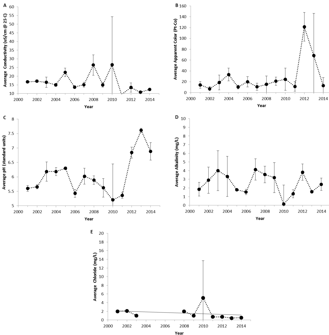
Figure 4. The annual average values of water quality indicators of Pine Lake, 2001-2014. (A) Specific lab conductivity @ 25 C, (B) apparent color, (C) pH, (D) total alkalinity, and (E) chloride. Vertical bars represent one standard deviation of the mean. Significant trends ( P \leq 0.05 ) are noted with a trend line.
