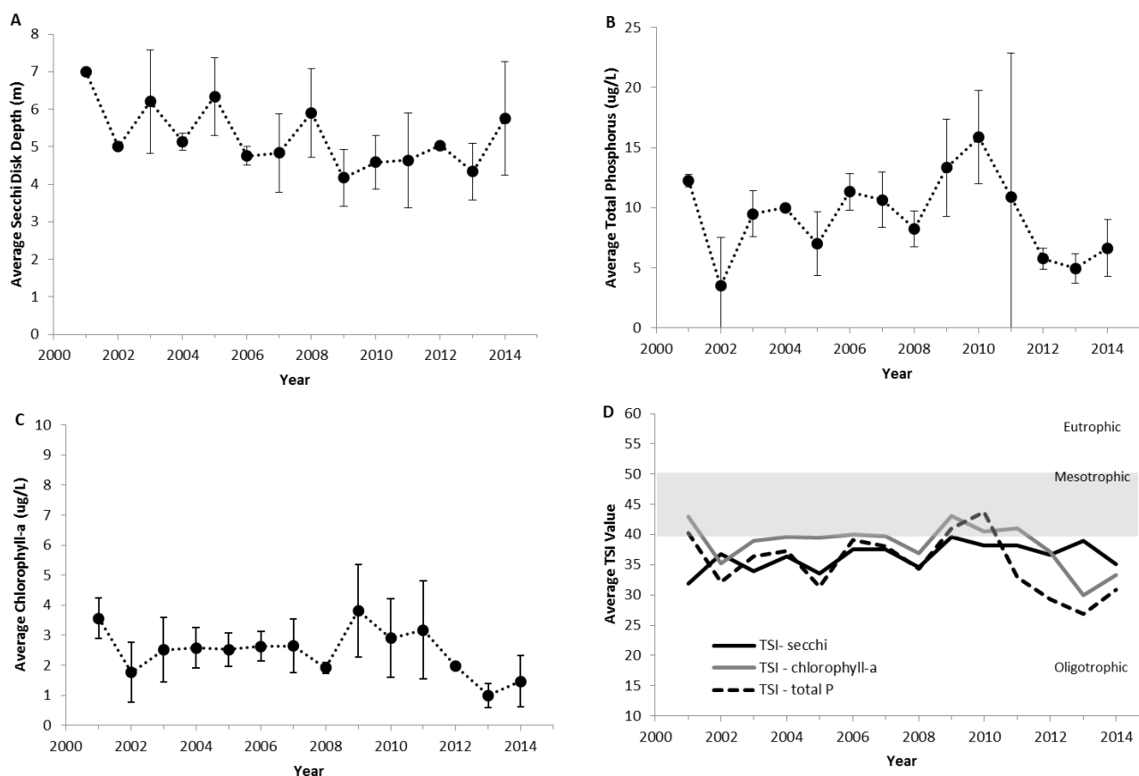
Figure 3. The annual average values of epilimnetic trophic indicators of Pine Lake, 2001-2014. (A) Secchi disk transparency, (B) total phosphorus concentration, (C) chlorophyll-a concentration, and (D) Carlson's Trophic Status Index. Vertical bars represent one standard deviation of the mean. Significant trends ( P \leq 0.05 ) are noted with a trend line.
