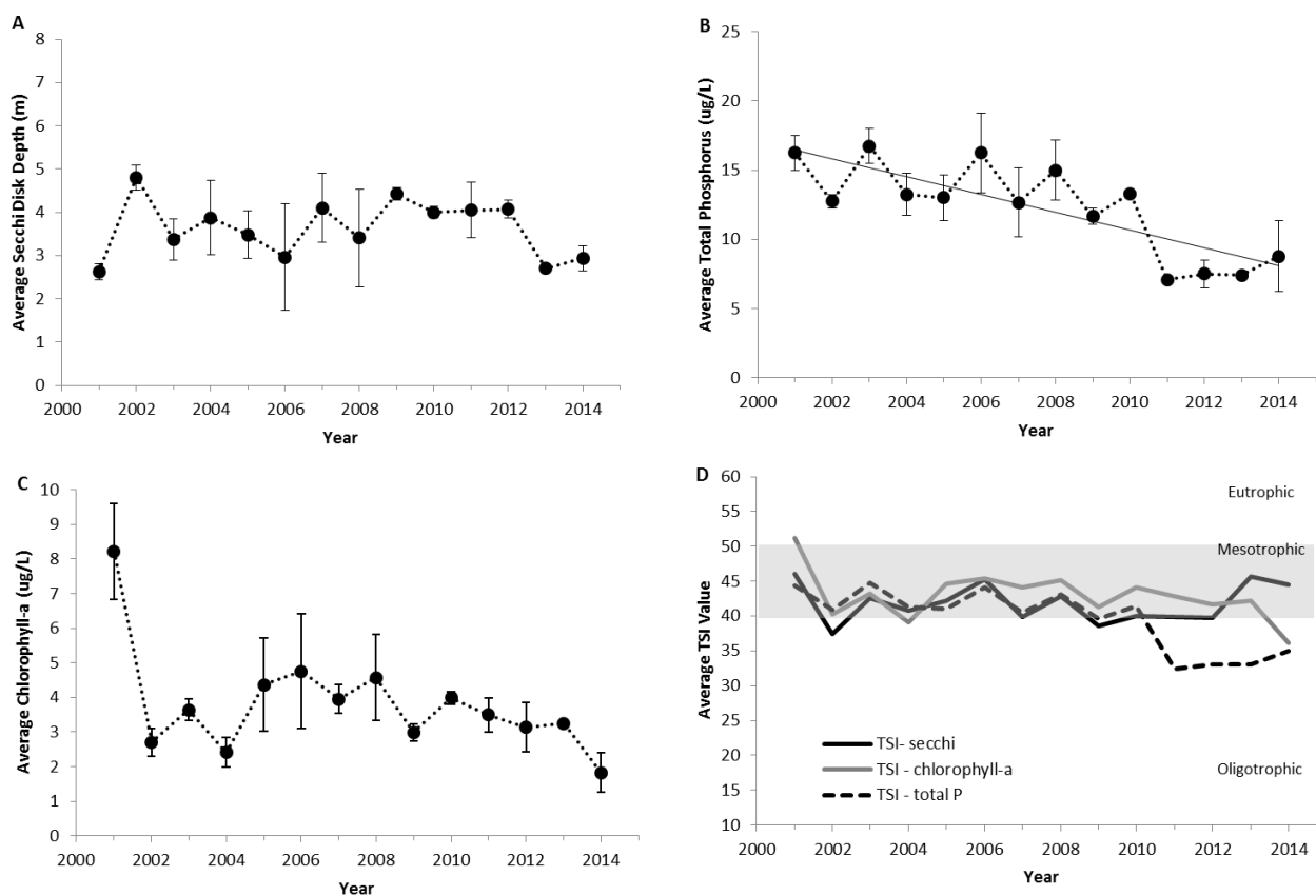
Figure 3. The annual average values of epilimnetic trophic indicators of Rich Lake, 2001-2014. (A) Secchi disk transparency, (B) total phosphorus concentration, (C) chlorophyll-a concentration, and (D) Carlson's Trophic Status Index. Vertical bars represent one standard deviation of the mean. Significant trends ( P\leq 0.05 ) are noted with a trend line.
