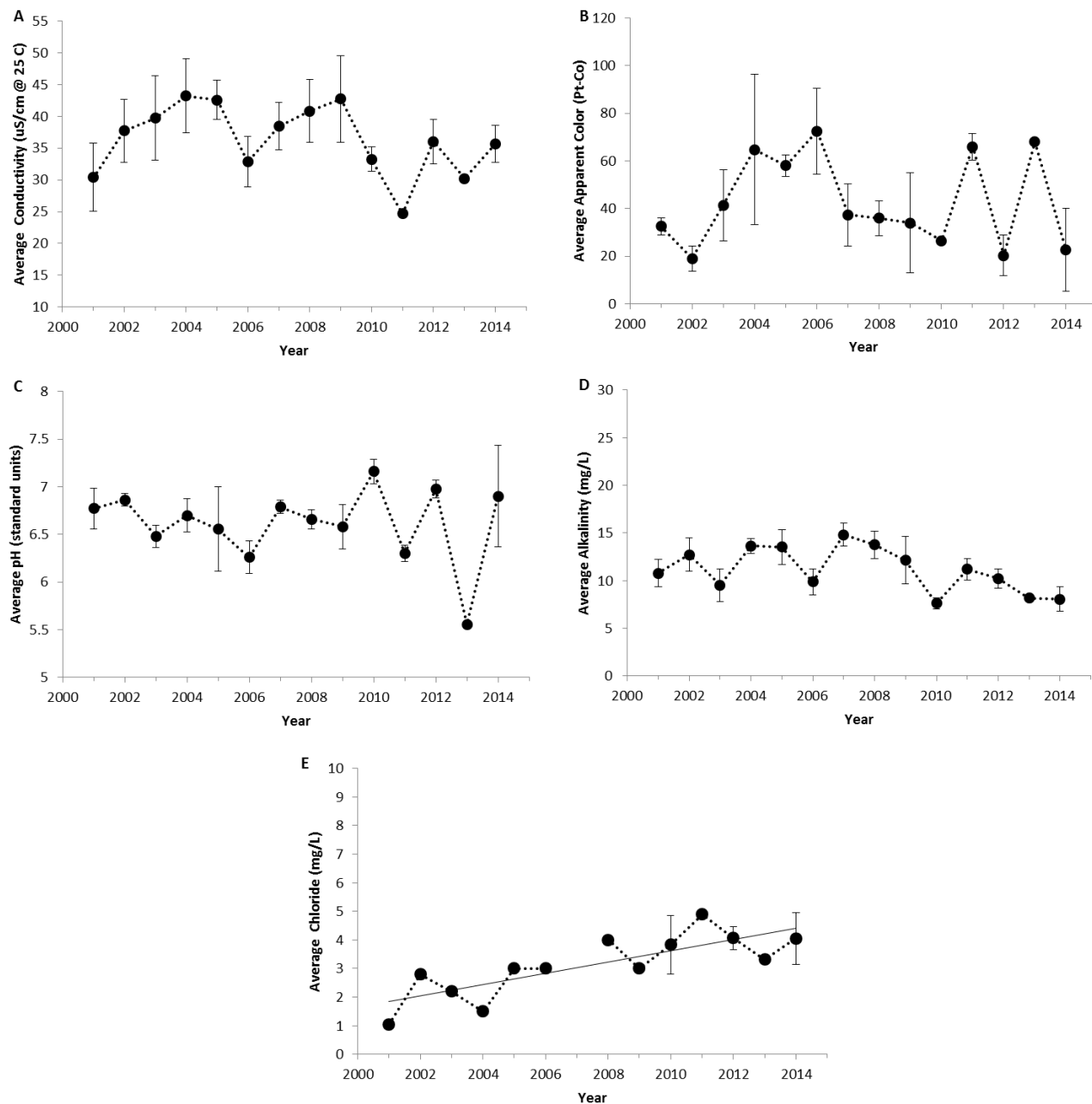
Figure 4. The annual average values of water quality indicators of Rich Lake, 2001-2014. (A) Specific lab conductivity @ 25 C, (B) apparent color, (C) pH, (D) total alkalinity, and (E) chloride. Vertical bars represent one standard deviation of the mean. Significant trends ( P \leq 0.05 ) are noted with a trend line.
