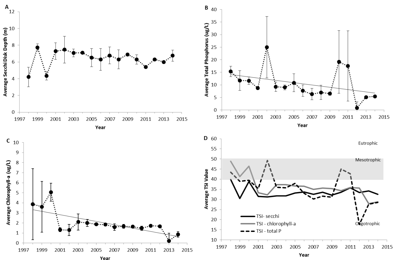
Figure 3. The annual average values of epilimnetic trophic indicators of Silver Lake, 1998-2014. (A) Secchi disk transparency, (B) total phosphorus concentration, (C) chlorophyll-a concentration, and (D) Carlson's Trophic Status Index. Vertical bars represent one standard deviation of the mean. Significant trends ( P\leq 0.05 ) are noted with a trend line.
