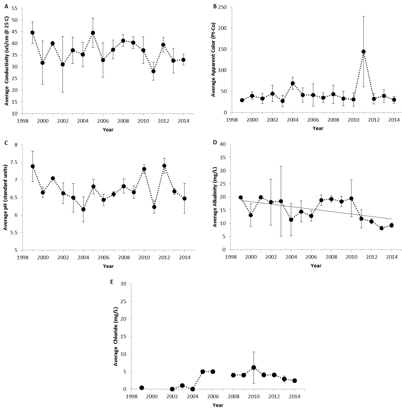
Figure 4. The annual average values of water quality indicators of Stony Creek Ponds, 1998-2014. (A) Specific lab conductivity @ 25 C, (B) apparent color, (C) pH, (D) total alkalinity, and (E) chloride. Vertical bars represent one standard deviation of the mean. Significant trends ( P \leq 0.05 ) are noted with a trend line.
