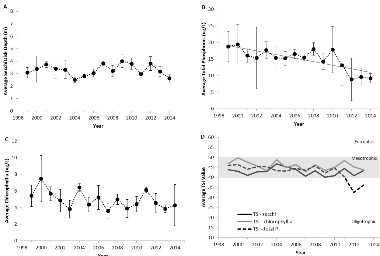
Figure 3. The annual average values of epilimnetic trophic indicators of Stony Creek Ponds, 1998-2014. (A) Secchi disk transparency, (B) total phosphorus concentration, (C) chlorophyll-a concentration, and (D) Carlson's Trophic Status Index. Vertical bars represent one standard deviation of the mean. Significant trends ( P \leq 0.05 ) are noted with a trend line.
